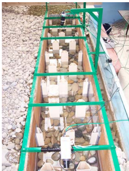
Figure 32. Photo de la configuration 1
